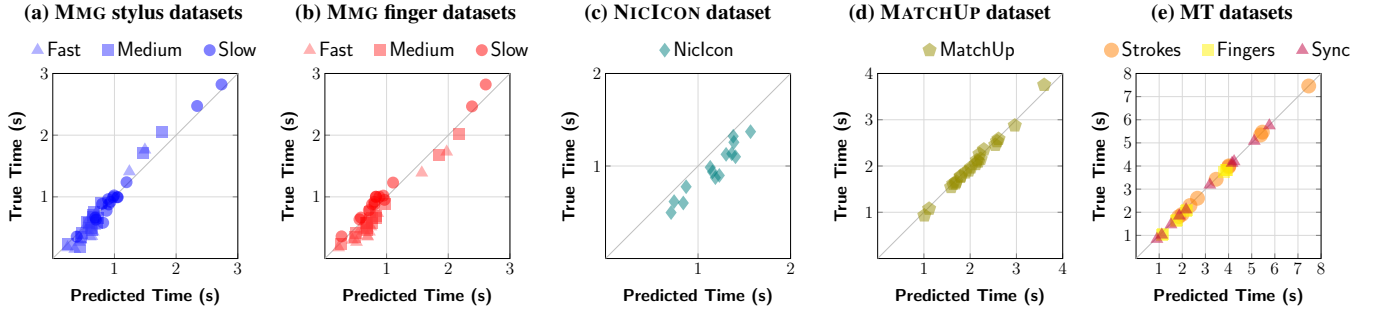
Figure 7. Production times ( \hat{t}_M ) predicted by GATO vs. groundtruth ( t_{True} ), averaged on a per-gesture basis.
